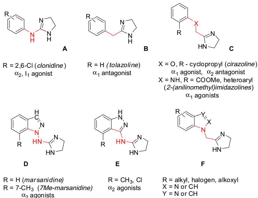
Figure 1. Structures of \alpha -adrenergic ligands A–C and their analogues D–F with partially restricted conformational freedom.
