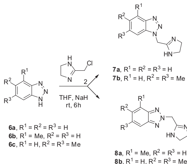
Scheme 2. Preparation of benzotriazol-1-yl derivatives 7a,b and benzotriazol-2-yl derivatives 8a,b .
