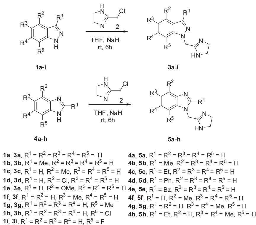
Scheme 1. Preparation of indazol-1-yl derivatives 3a–i and benzimidazol-1-yl derivatives 5a–h .
